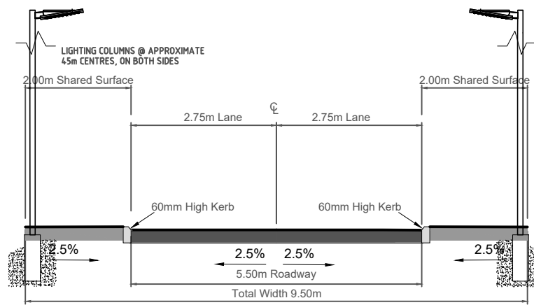
Typical Section Thru' 5.5m Side Road (Scale 1:50)
