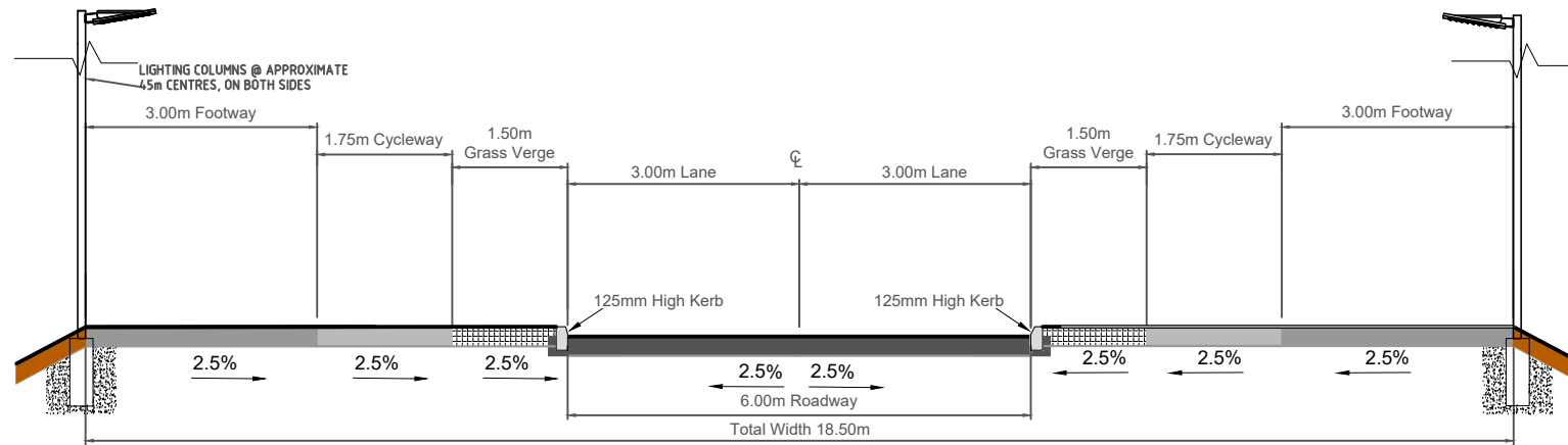
Typical Section Thru' 6.0m Main Road 01 (Scale 1:50)
