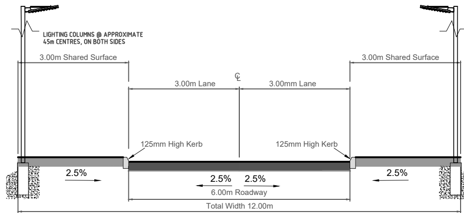
Typical Section Thru' 6.0m Main Road 02 (Scale 1:50)
