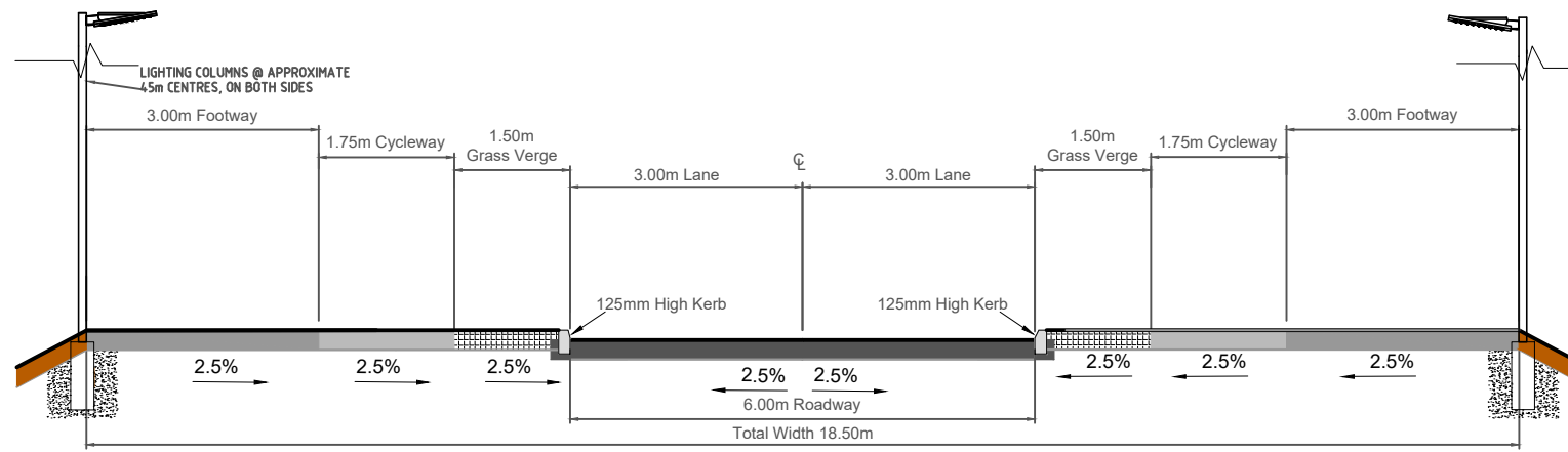
Typical Section Thru' 6.0m Northern Spine Road (Blandcrest Main Road 1) (Scale 1 : 50)
