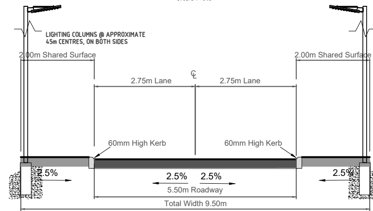
Typical Section Thru' 5.5m (SR Type Roads) (Scale 1 : 50)
