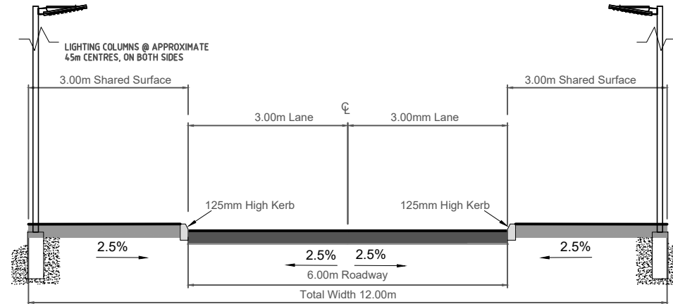
Typical Section Thru' 6.0m (MR 02) (Scale 1 : 50)
