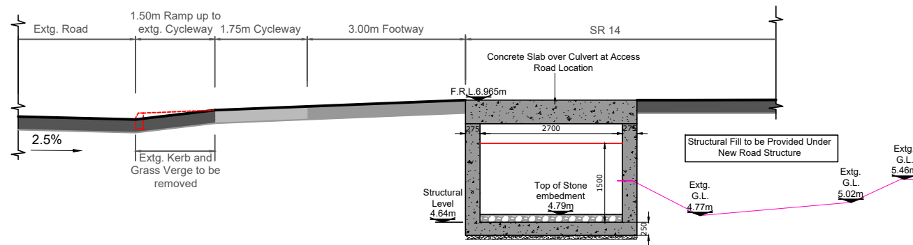
Section at Culvert Crossing at SR 14 (SR 15 Similar arrangement) (Scale 1 : 50)
