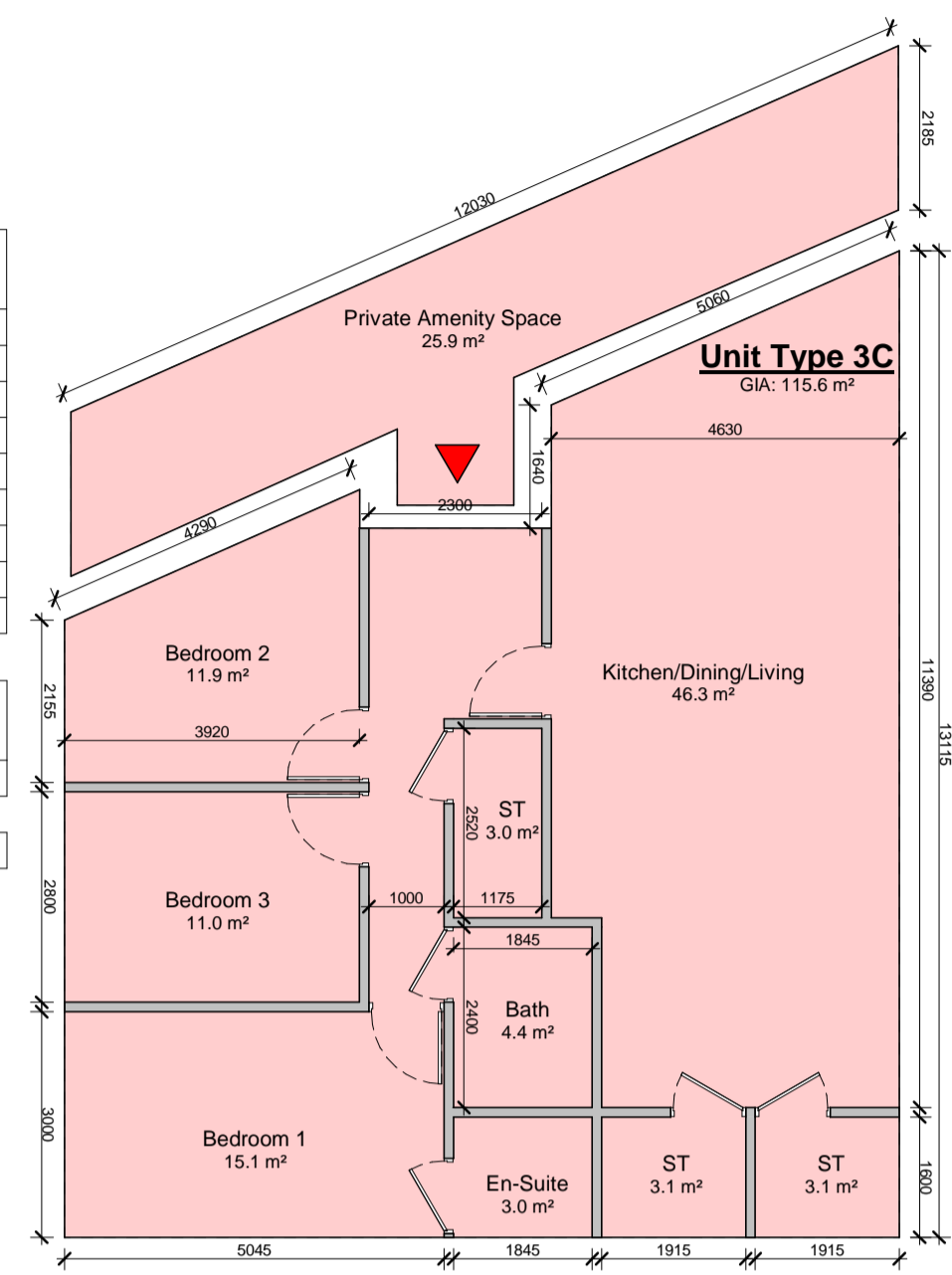
3 Apartment Type 3C 1 : 100
