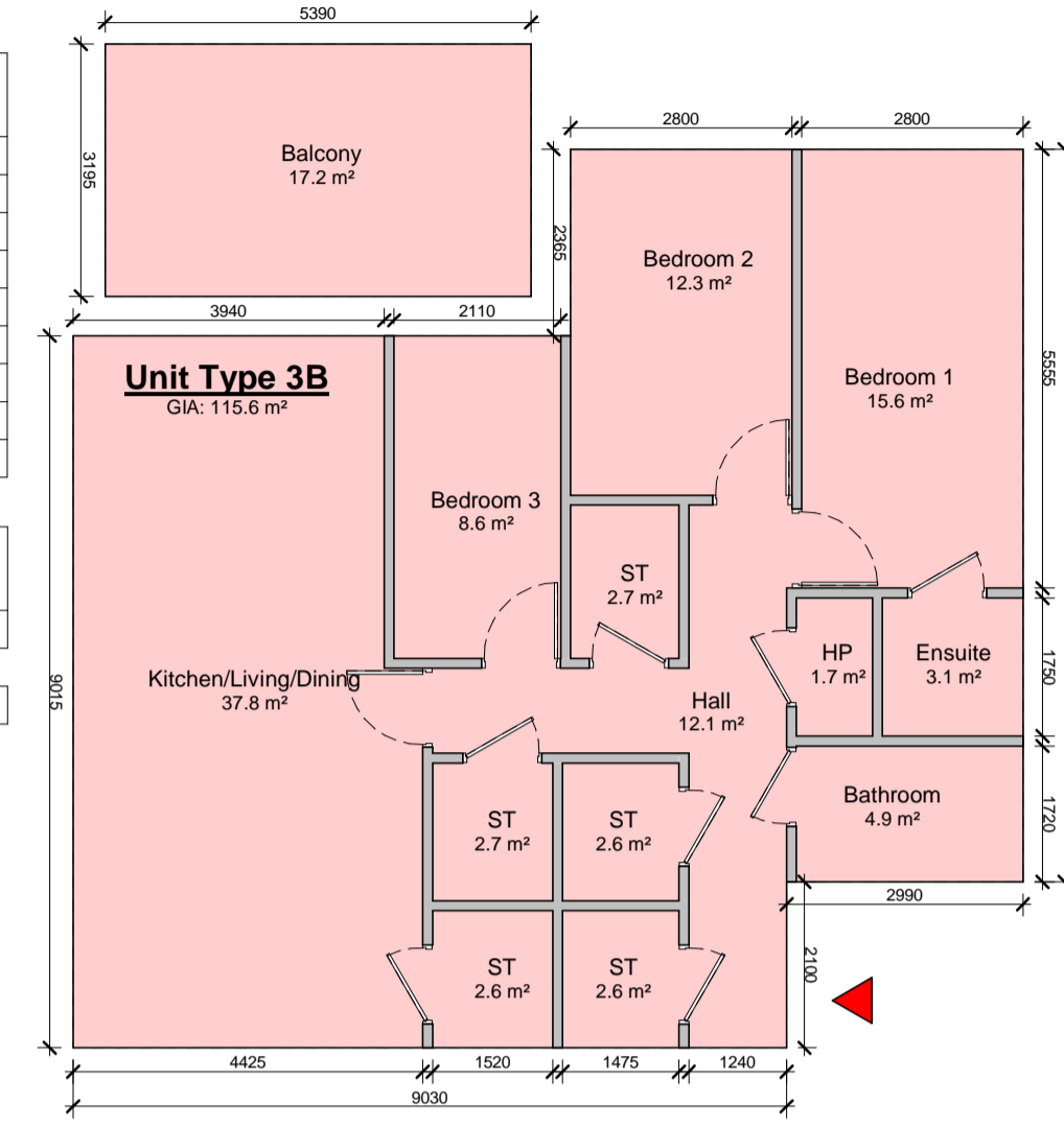
2 Apartment Type 3B 1 : 100
