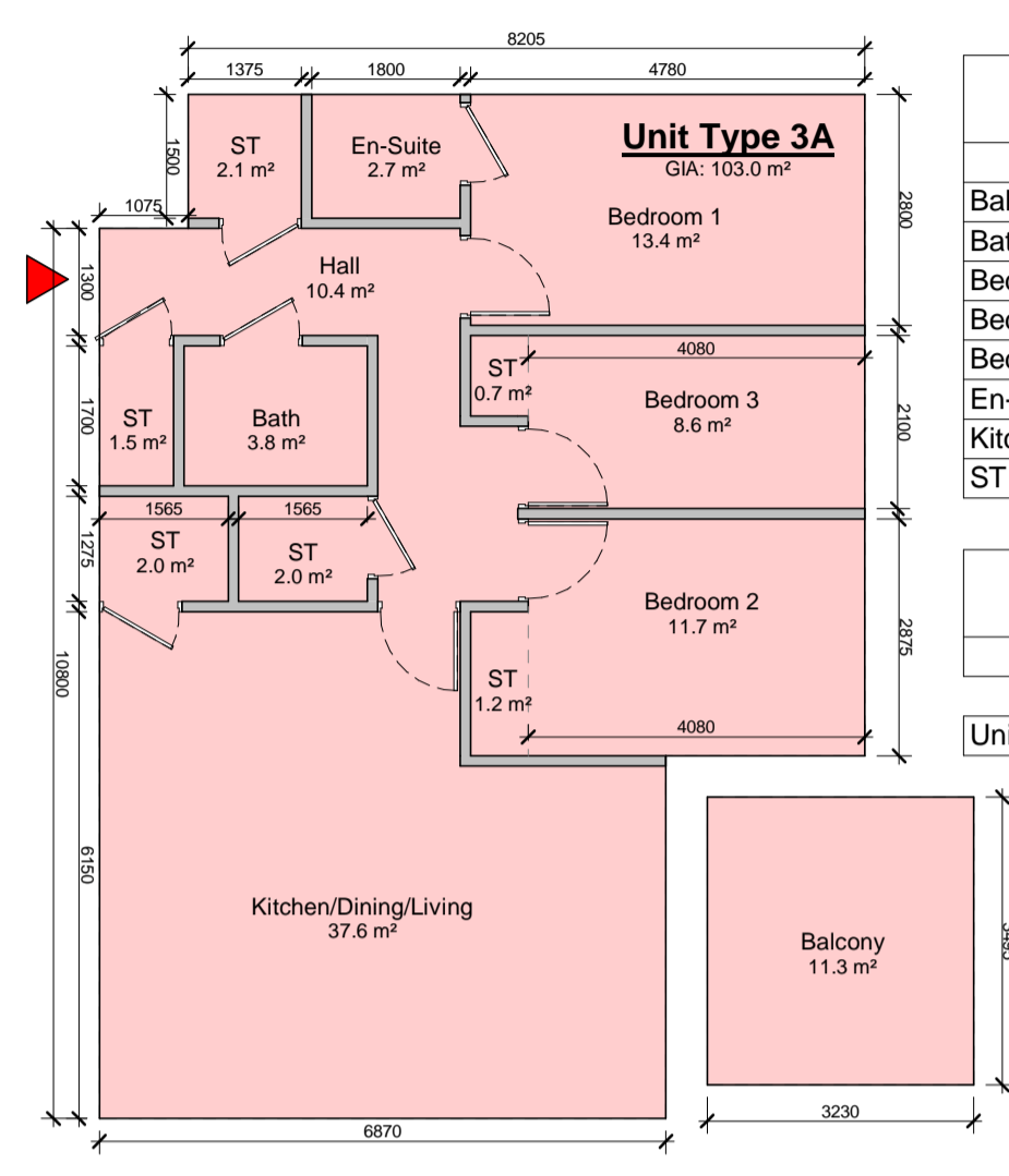
1 Apartment Type 3A 1 : 100
