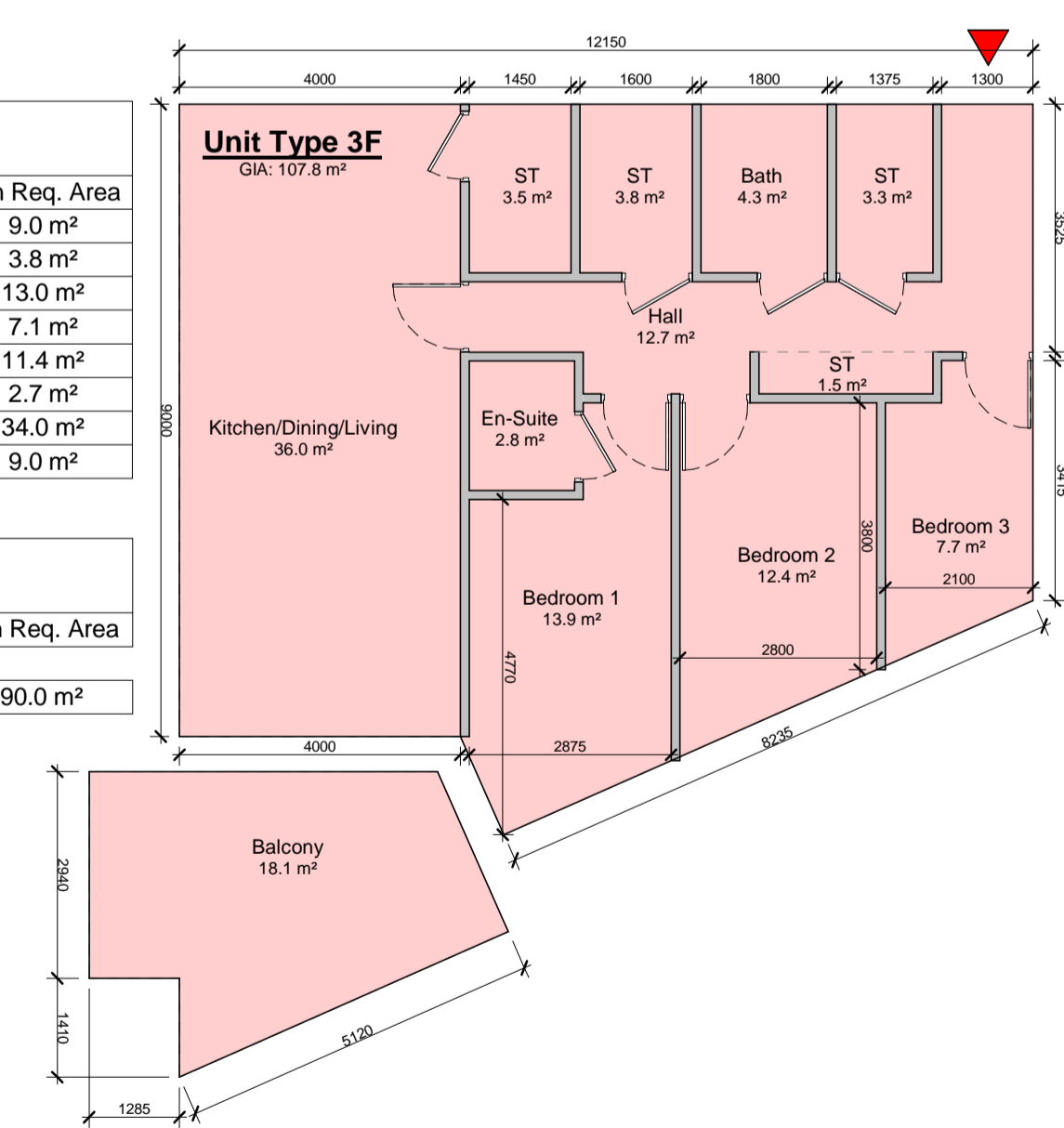
6 Apartment Type 3F 1 : 100
