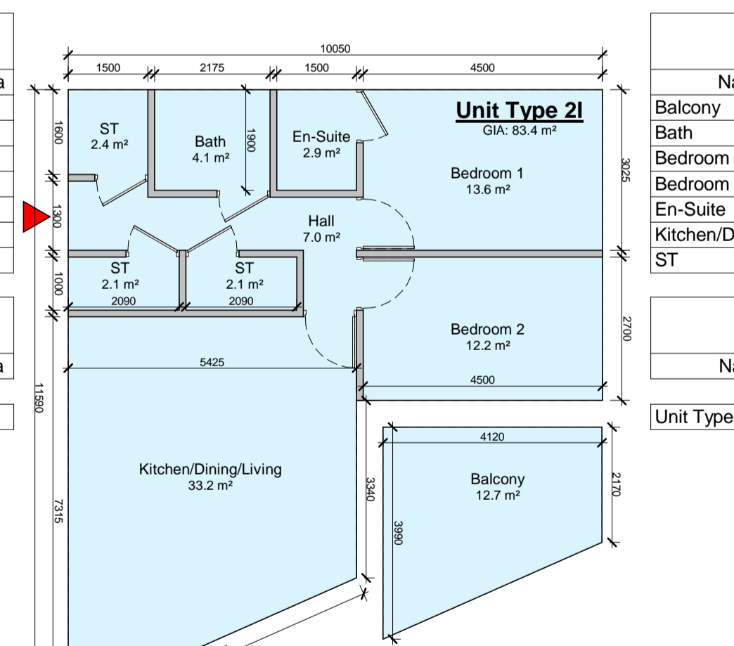
9 Apartment Type 2i 1 : 100
