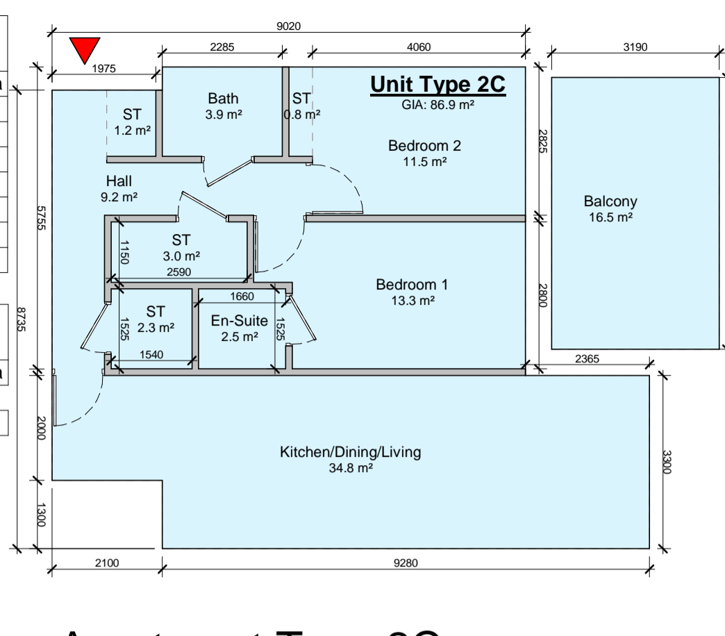
3 Apartment Type 2C 1 : 100
