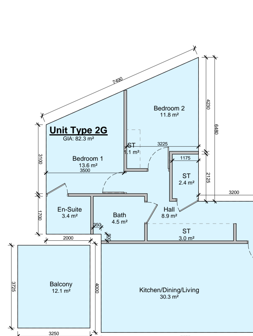
7 Apartment Type 2G 1 : 100
