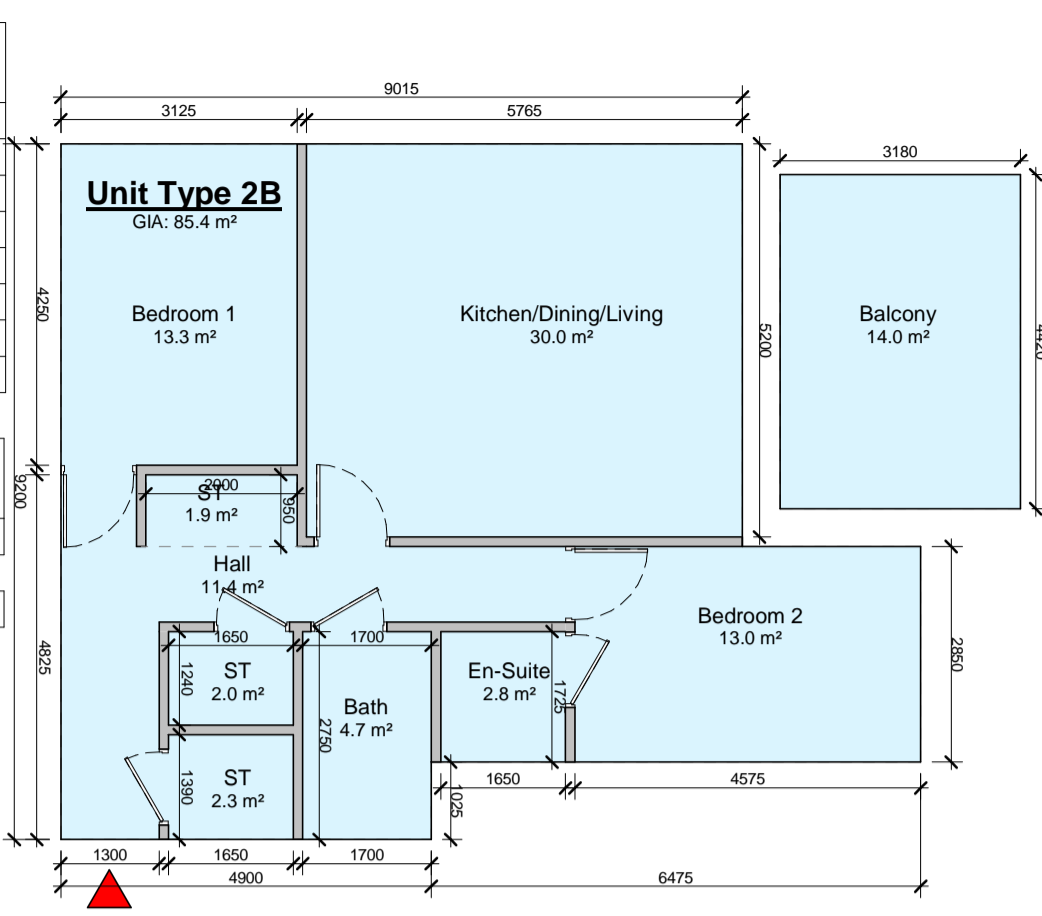
2 Apartment Type 2B 1 : 100
