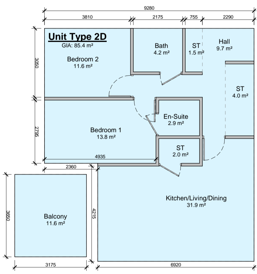
4 Apartment Type 2D 1 : 100
