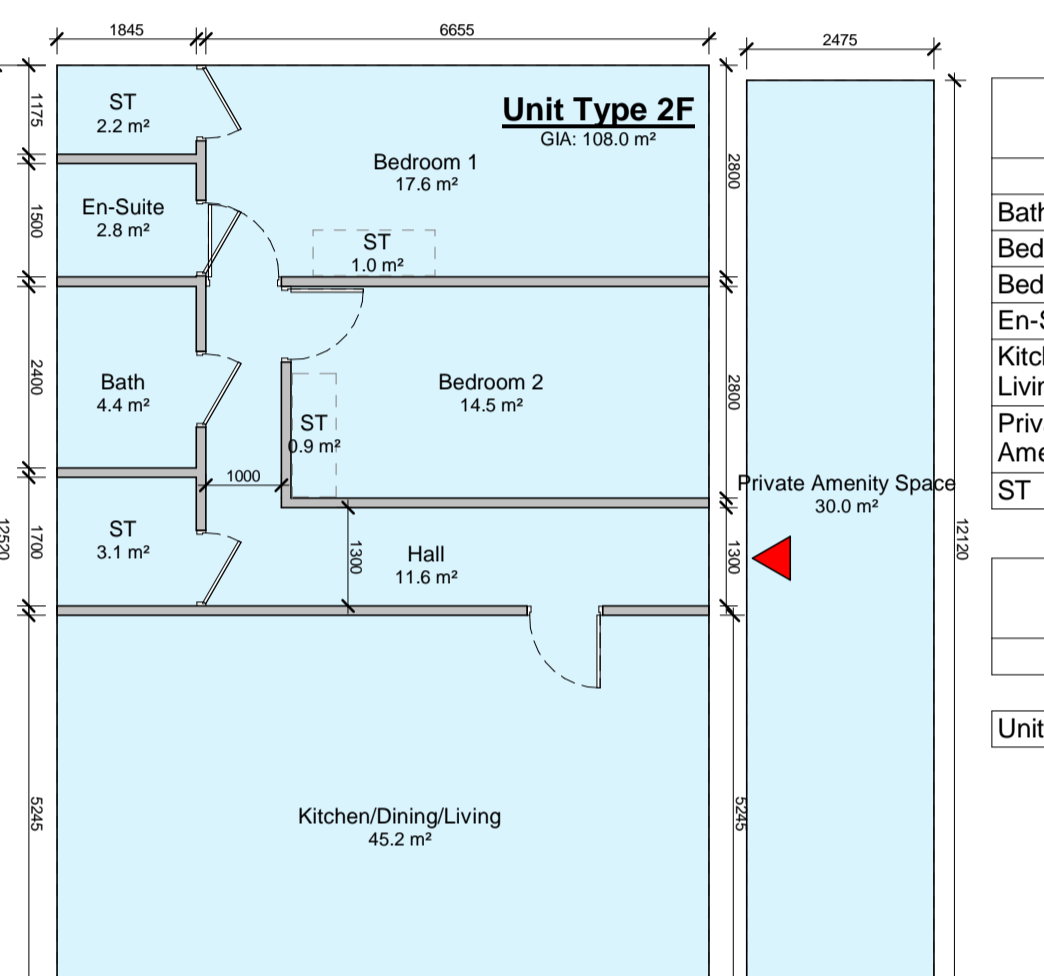
6 Apartment Type 2F 1 : 100
