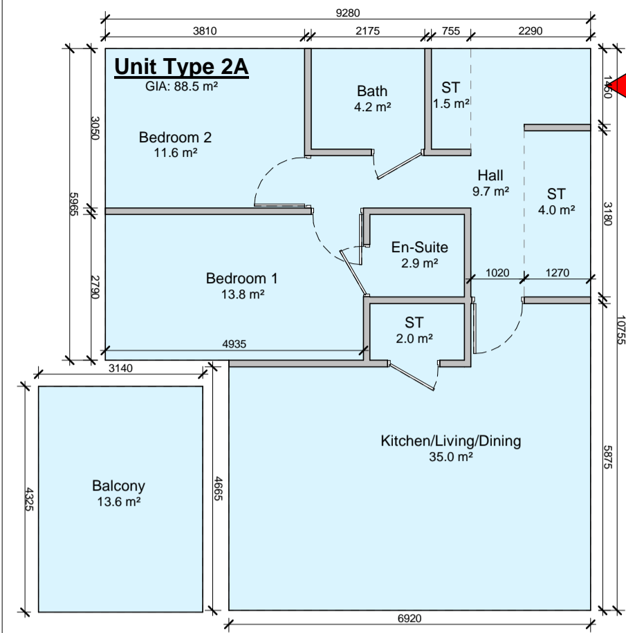
1 Apartment Type 2A 1 : 100
