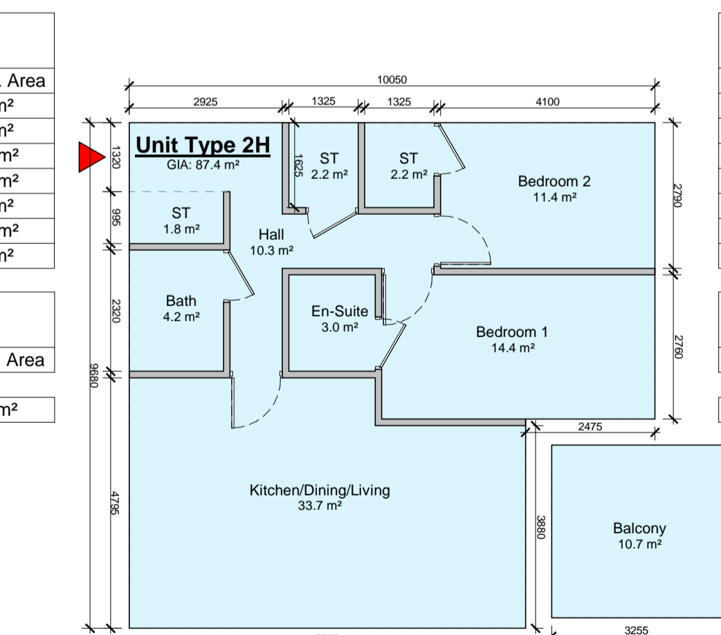
8 Apartment Type 2H 1 : 100
